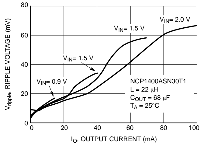
Figure 30. NCP1400ASN30T1 Ripple Voltage vs. Output Current
