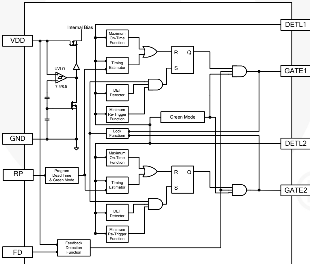
Figure 2. Block Diagram
