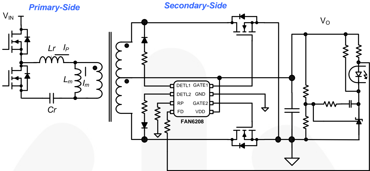
Figure 1. Typical Application
