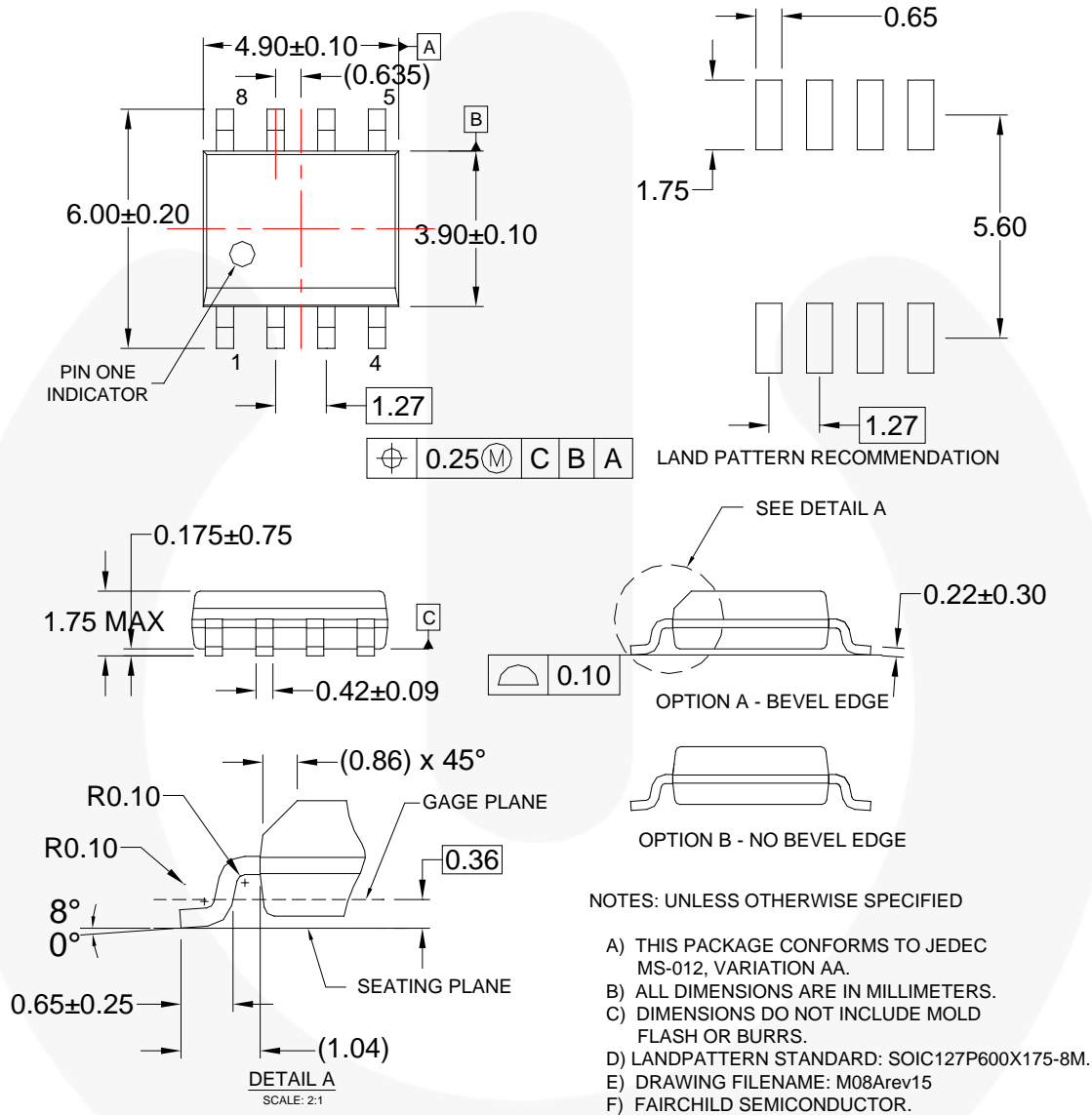
Figure 45. 8-Lead, SOIC, JEDEC MS-012, .150-Inch Narrow Body
