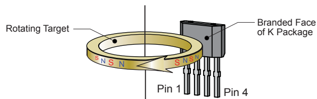
Figure 2. This left-to-right (pin 1 to pin 4) direction of target rotation results in a high output signal when a target north pole is nearest the face of the device (see figure 3). A right-to-left (pin 4 to pin 1) rotation inverts the output signal polarity.
