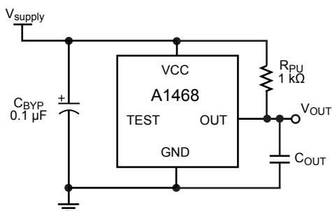
Figure 6. Typical Application Diagram
