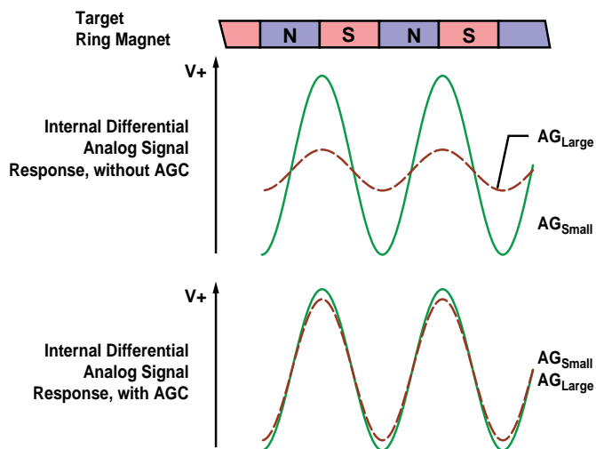
Figure 4. Automatic Gain Control (AGC). The AGC function corrects for variances in the air gap. Differences in the air gap affect the magnetic gradient, but AGC prevents that from affecting device performance, as shown in the lowest panel.
