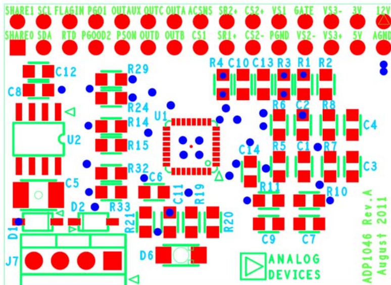
Figure 81 - Top Layer
