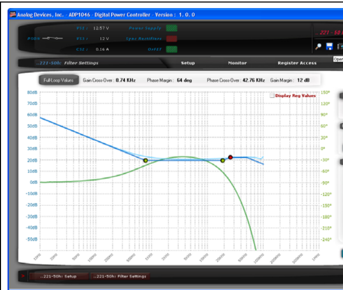
Figure 41 – Digital compensation for Light Load mode (DCM)
