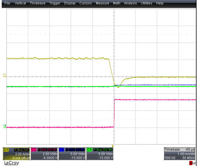
Figure 58 – Output reverse current protection, threshold 'B' Red trace: OrFET gate signal Green and Blue trace: Output voltages of two power supplies Yellow trace: Load current
