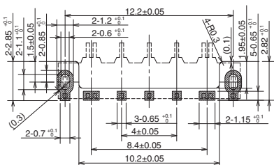
PCB Mating Dimensions (TOP VIEW)
