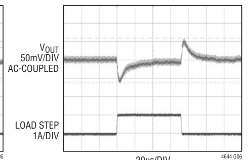
2.5V Output Transient Response
