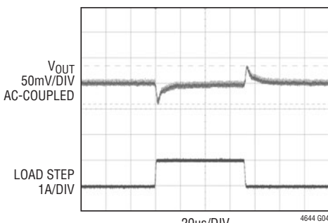
1.0V Output Transient Response
