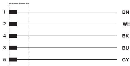
Contact assignment of the M12 connector
