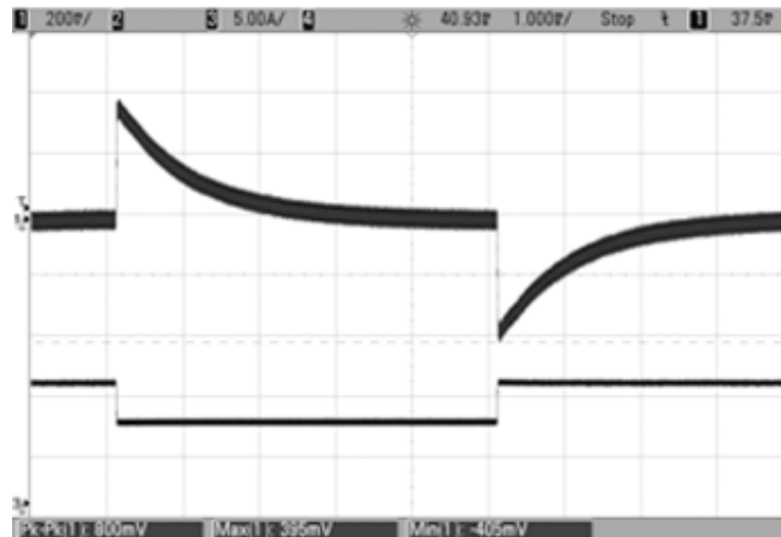
Step Load Transient Response (Vin = 48V, Vout = nom, Cload = 1µF || 10µF, Iout = 50 to 50% of full load, Ta = +25°C) Ch1 = Vout, Ch2 = Iout.
