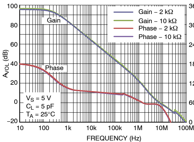
Figure 11. Open Loop Gain and Phase vs. Frequency @ V_S = 5\text{ V}
