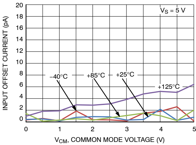
Figure 3. Input Offset Current vs. V_{CM}
