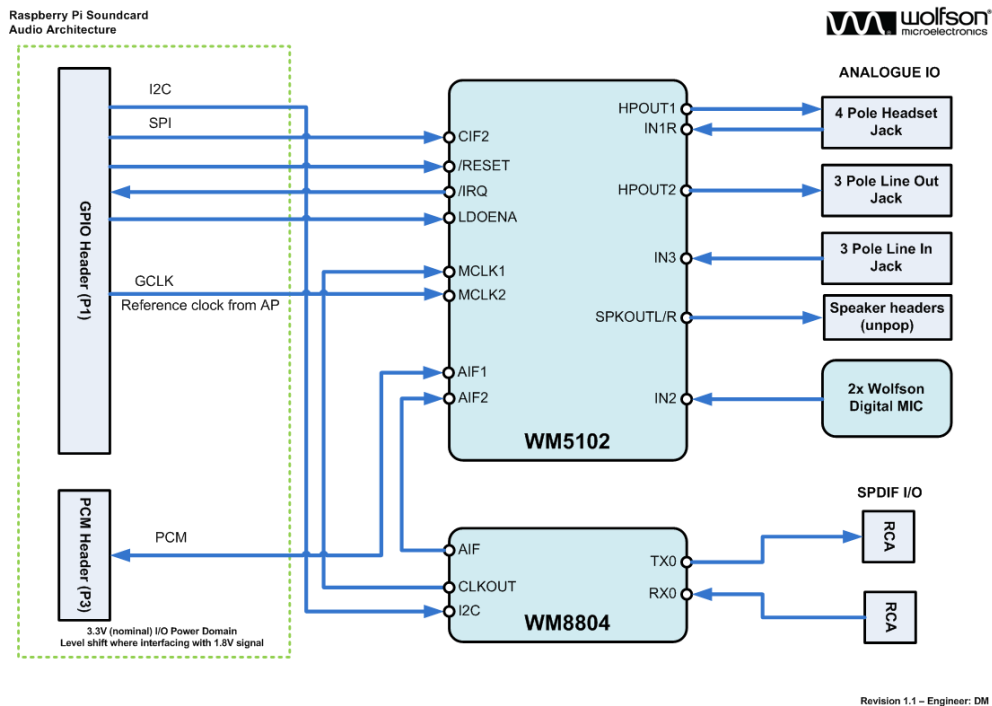
Diagram 4: Audio architecture of the Wolfson audio card
