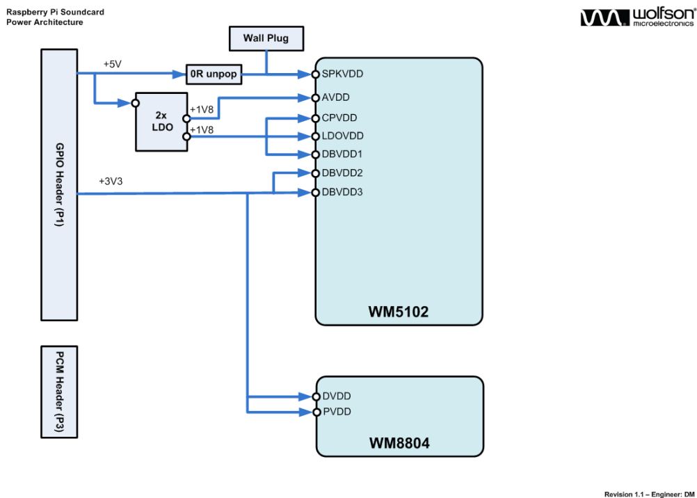
Diagram 5: Power management architecture of the Wolfson audio card
