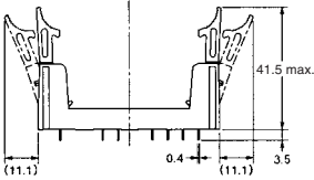
G7SA-4A2B Mounted
