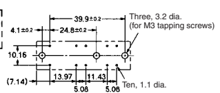
Mounting Hole Placement (Bottom View) (±0.1 tolerance)
