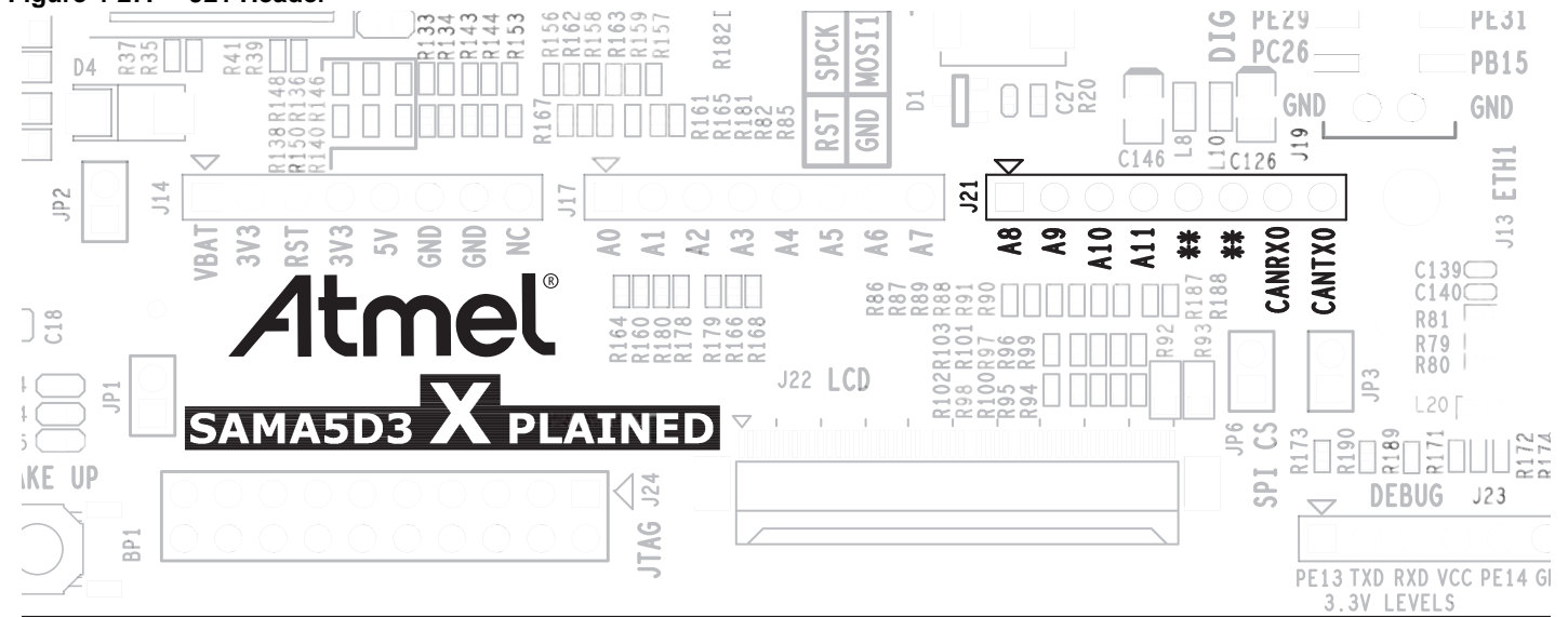
Figure 4-27. J21 Header
