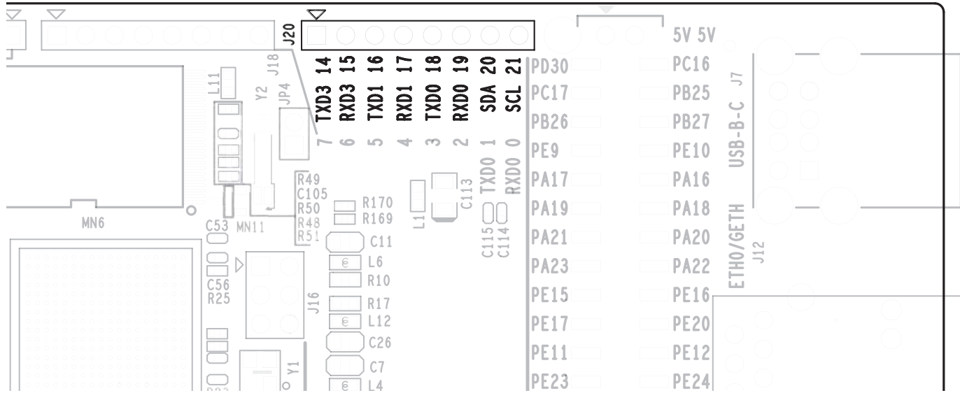
Figure 4-22. J20 Header
