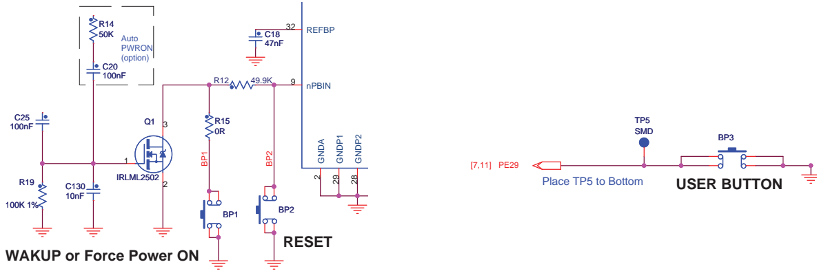
Figure 4-16. Pushbutton Schematic
