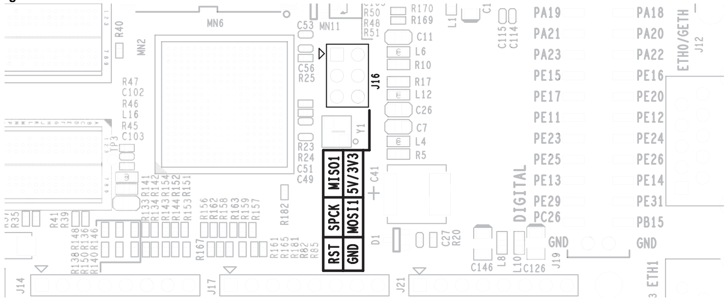
Figure 4-24. J16 Header
