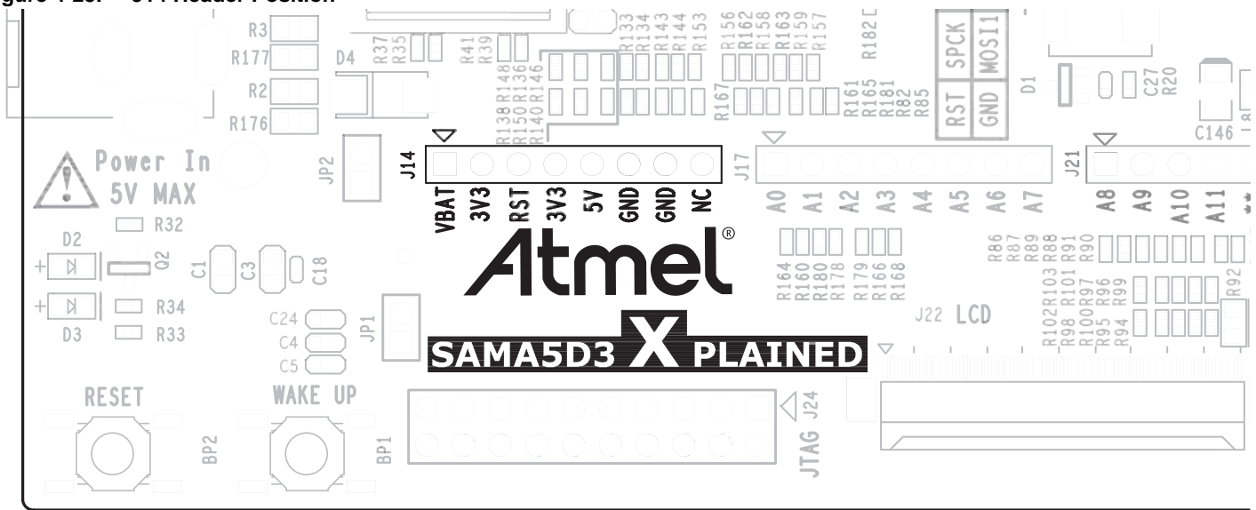
Figure 4-25. J14 Header Position
