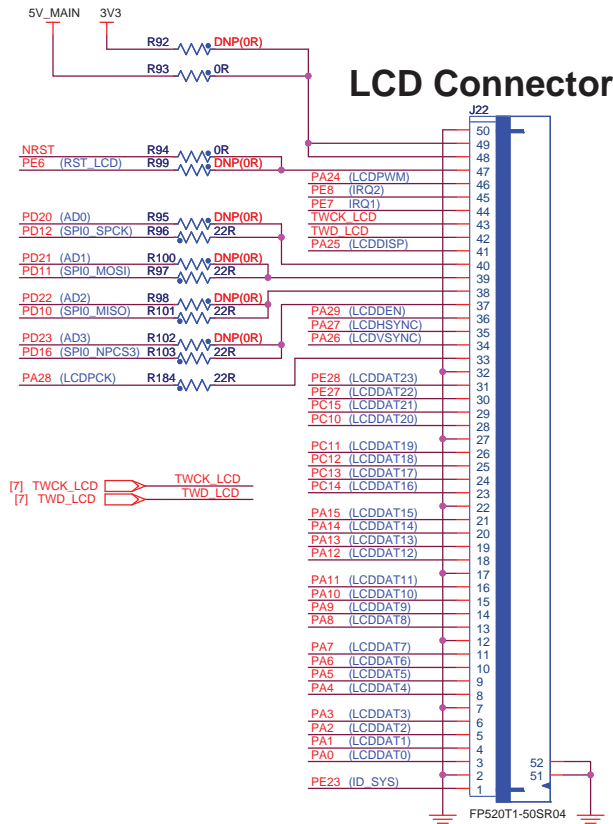
Figure 4-17. LCD Expansion Header Interface Schematic
