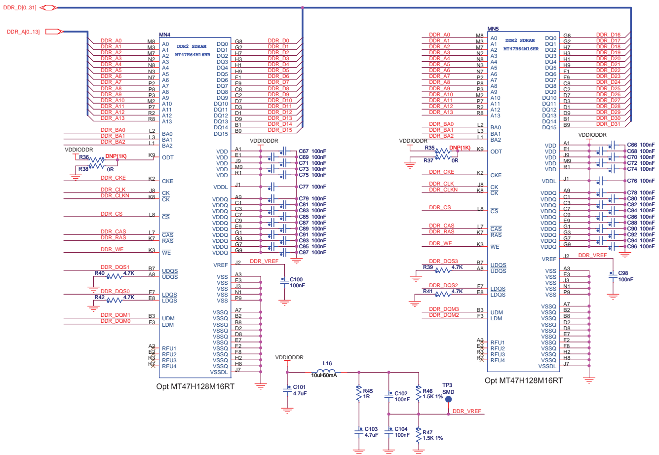
Figure 4-6. DDR2 Schematic
