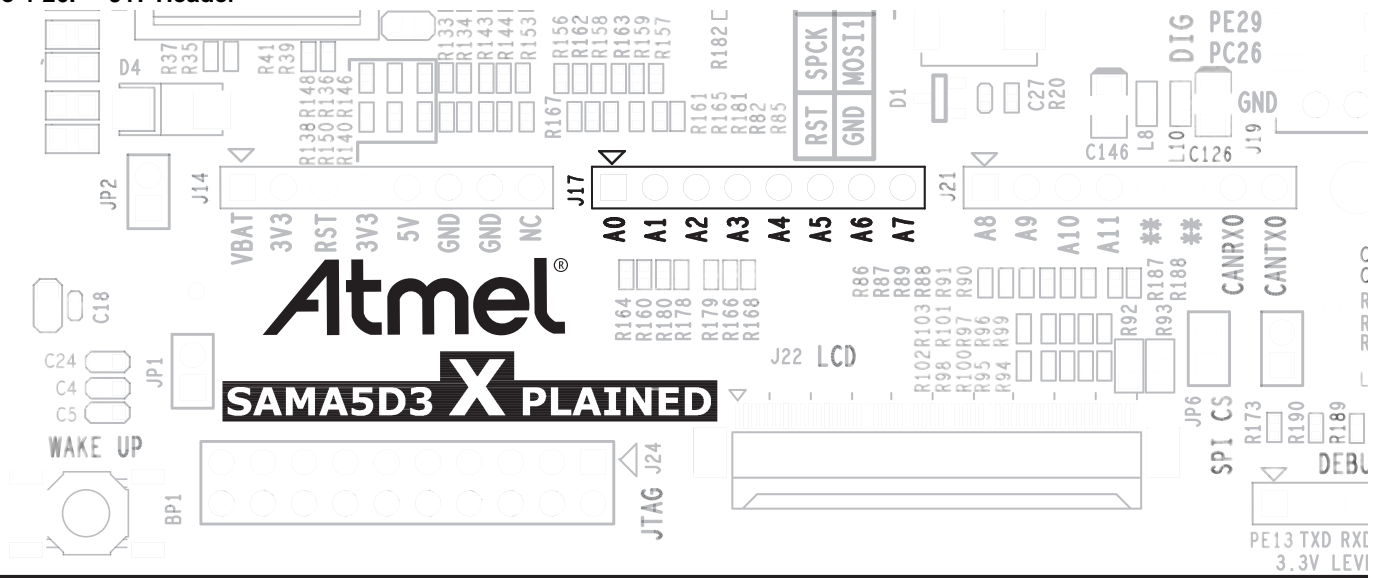
Figure 4-26. J17 Header
