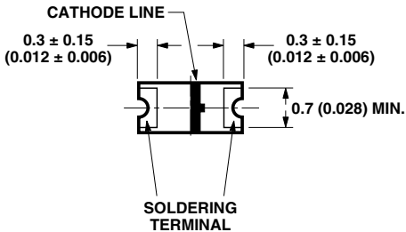
HSMx-C190
