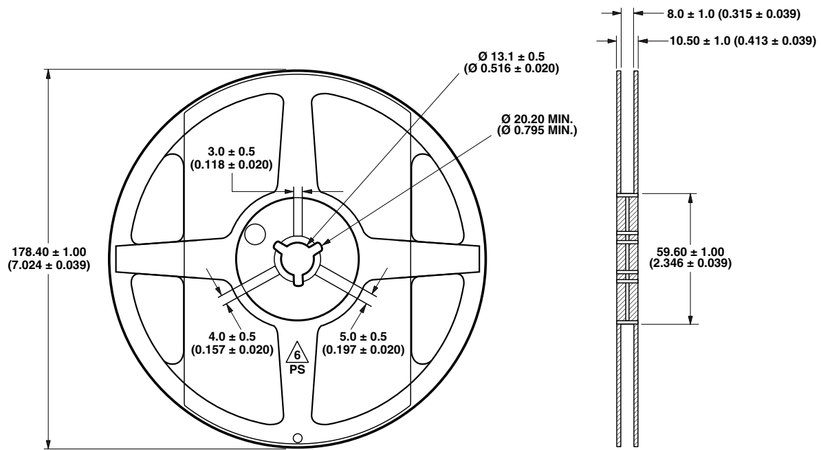
Figure 20. Reel dimensions.
