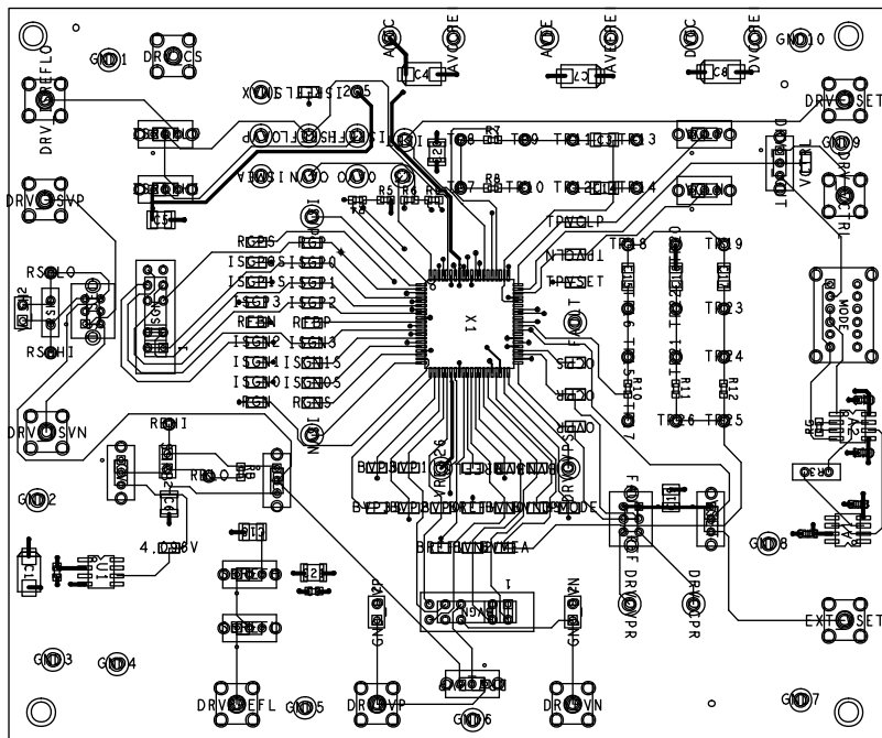
Figure 64. AD8450-EVALZ Primary Side Copper
