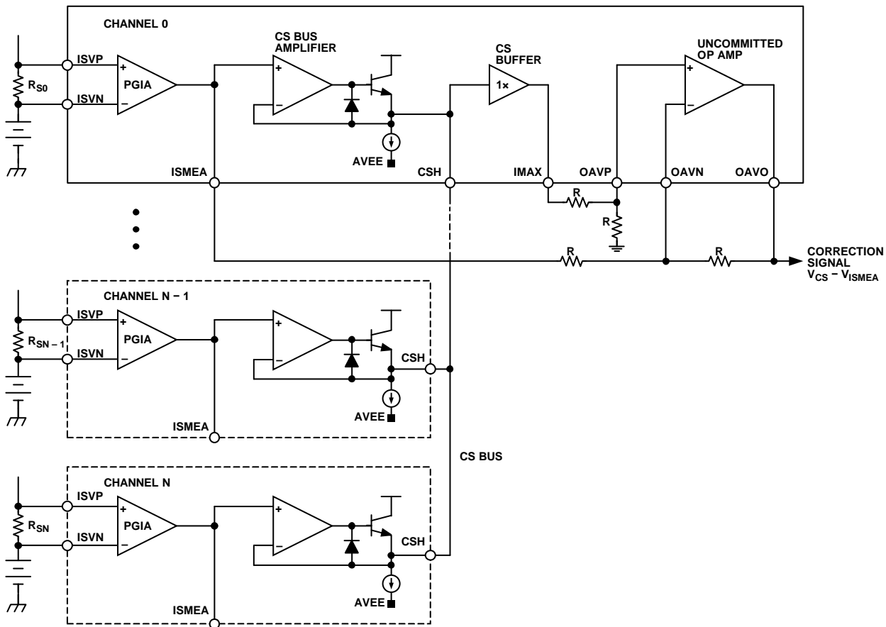
Figure 58. Functional Block Diagram of the Current Sharing Circuit
