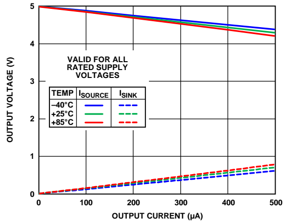
Figure 43. Output Voltage vs. Output Current at Three Temperatures
