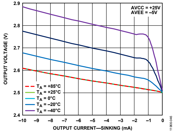
Figure 46. Output Voltage vs. Output Current (Sinking) over Temperature
