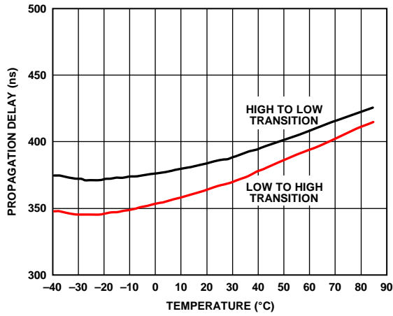
Figure 40. Propagation Delay vs. Temperature
