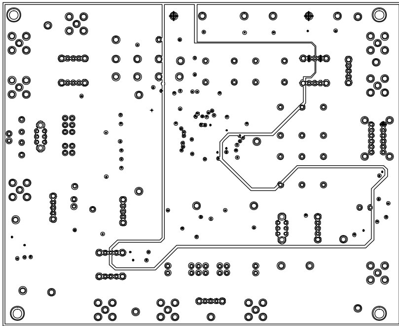
Figure 66. AD8450-EVALZ Power Plane
