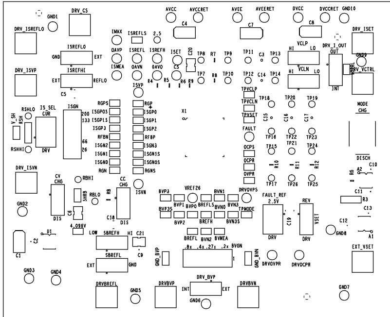
Figure 63. Top Silkscreen of the AD8450-EVALZ
