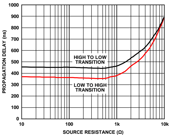
Figure 42. Propagation Delay vs. Source Resistance
