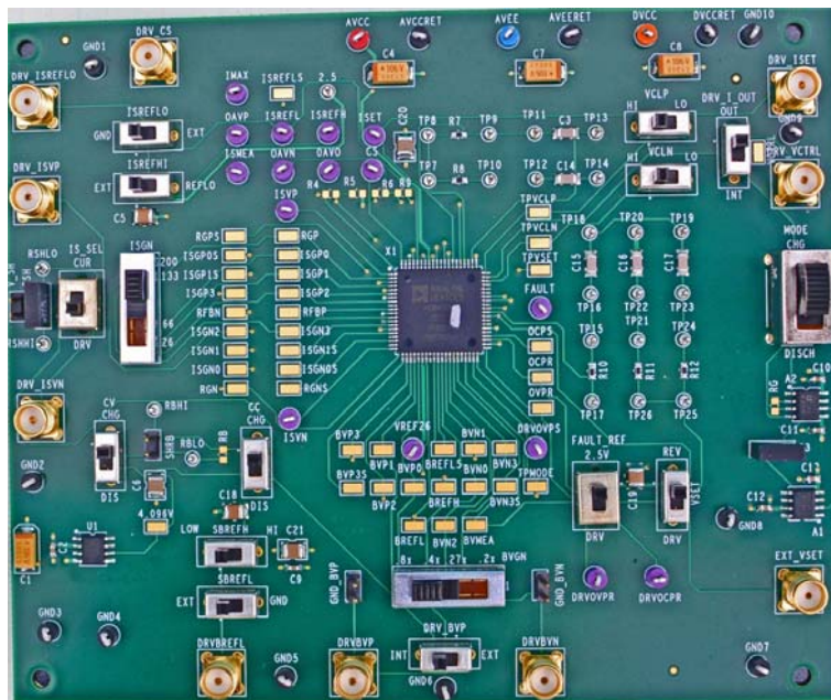
Figure 61. Photograph of the AD8450-EVALZ
