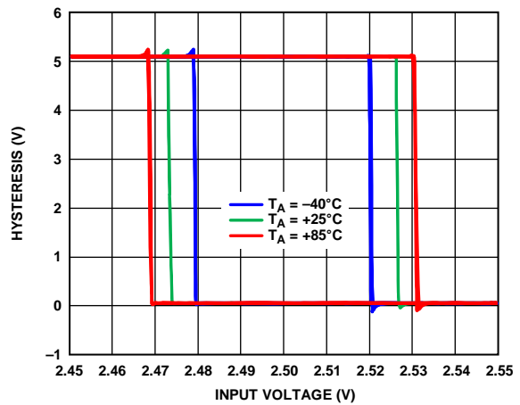
Figure 44. Comparator Transfer Function at Three Temperatures
