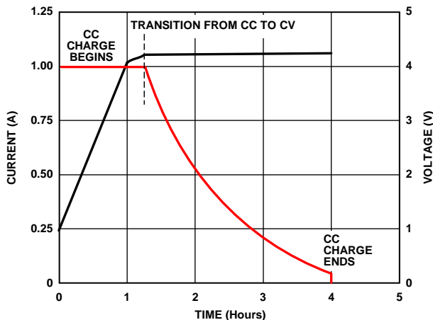
Figure 54. Representative Constant Current to Constant Voltage Transition Near the End of a Battery Charging Cycle
