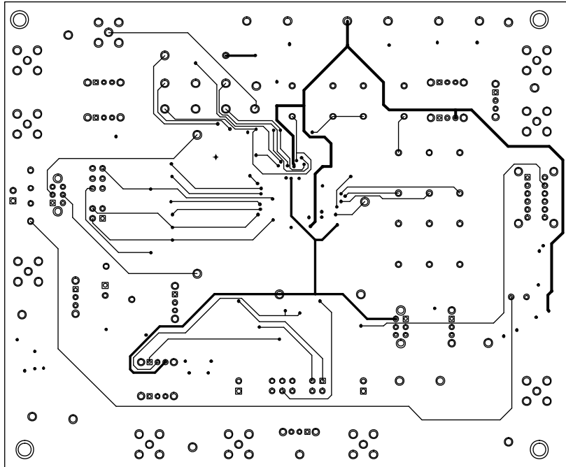
Figure 65. AD8450-EVALZ Secondary Side Copper
