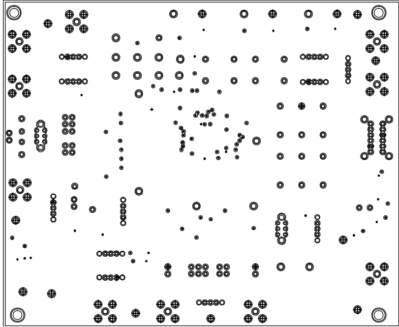
Figure 67. AD8450-EVALZ Ground Plane
