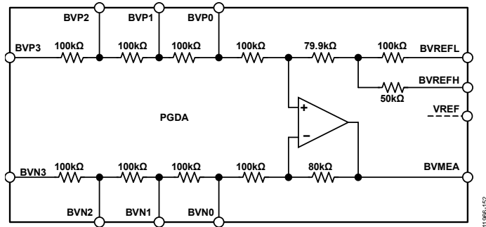
Figure 52. PGDA Simplified Block Diagram
