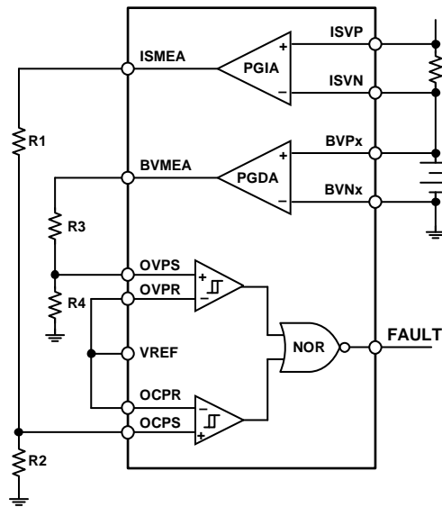
Figure 56. OVP and OCP Comparator Configuration Using the Internal Reference
