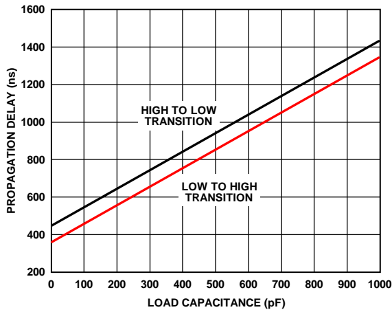
Figure 41. Propagation Delay vs. Load Capacitance
