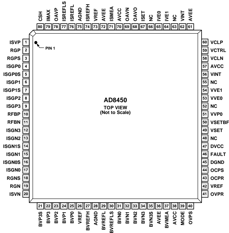
Figure 2. Pin Configuration
