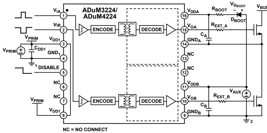
NC = NO CONNECT 1 GND 1 IS CONNECTED TO THE PRIMARY SIDE GROUND, ISOLATED FROM THE SECONDARY GROUND. 2 GND B IS CONNECTED TO THE SECONDARY SIDE GROUND, ISOLATED FROM THE PRIMARY GROUND.
