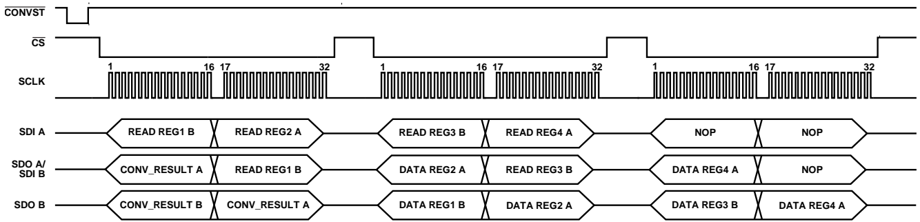
Figure 56. Multiple Register Read in a Two-Slave Daisy-Chain Mode Configuration
