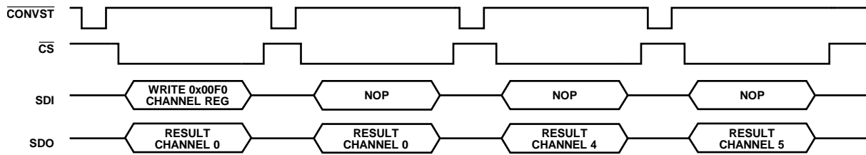
Figure 50. Channel Sequencer
