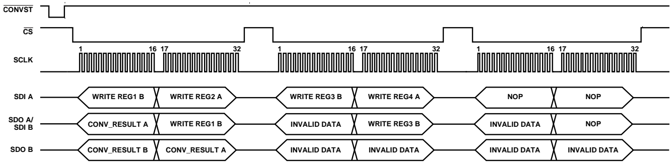
Figure 57. Multiple Register Write in a Two-Slave Daisy-Chain Mode Configuration
