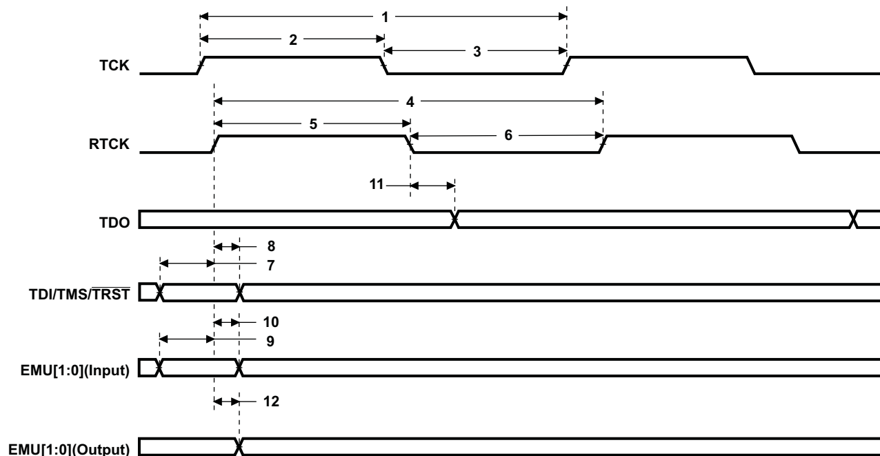
Figure 7-97. JTAG Test-Port Timing
