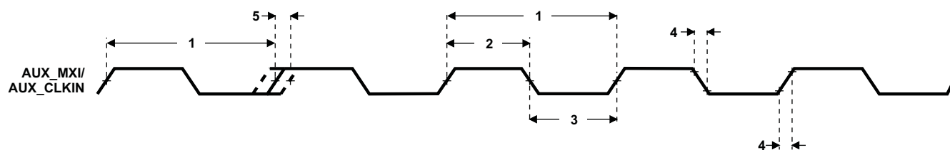
Figure 7-17. AUX_MXI/AUX_CLKIN Timing
