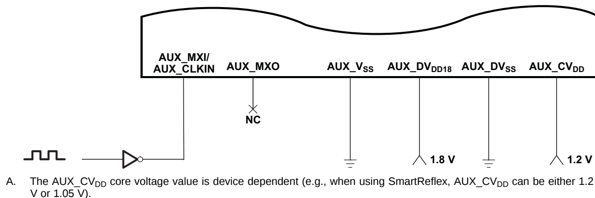
Figure 7-11. 1.8-V LVC MOS-Compatible Clock Input (A)
