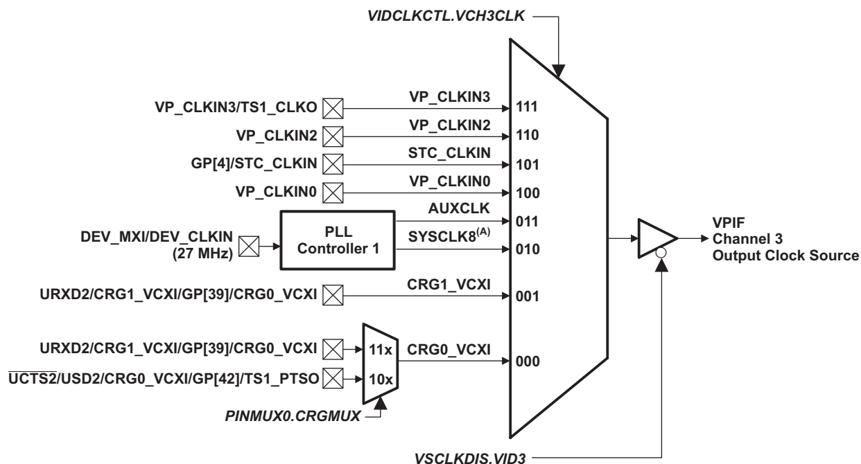
Figure 7-38. VPIF Display Channel 3 Source Clock Selection
