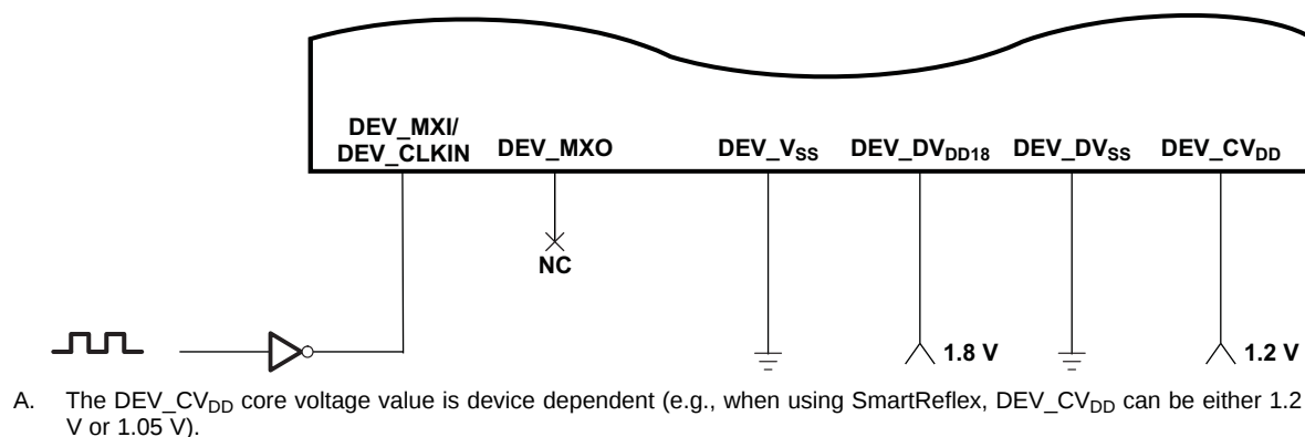
Figure 7-10. 1.8-V LVC MOS-Compatible Clock Input (A)
