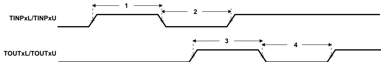
Figure 7-94. Timer Timing
