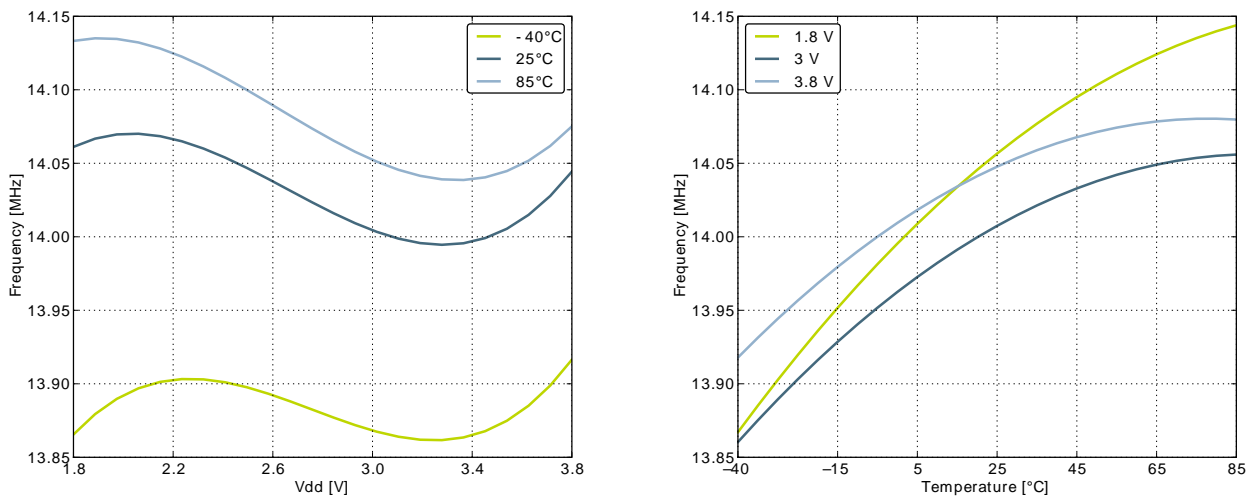
Figure 3.13. Calibrated HFRCO 21 MHz Band Frequency vs Supply Voltage and Temperature
