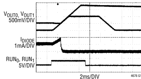
FIGURE 44 CIRCUIT AT 12\text{V}_{\text{IN}} , 77mΩ LOAD ON V OUT0 , 500Ω ON V OUT1 . V OUT1 PRE-BIASED THROUGH A DIODE. TON_RISE 0 = 3ms, TON_RISE 1 = 5.297ms, TOFF_DELAY 1 = 0ms, TOFF_DELAY 0 = 2.43ms, TOFF_FALL 1 = 5.328ms, TOFF_FALL 0 = 3ms, ON_OFF_CONFIG 1 = 0x1F ON_OFF_CONFIG 0 = 0x1E
