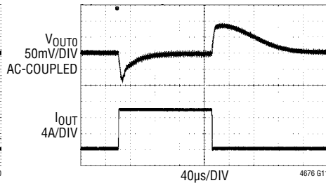
FIGURE 44 CIRCUIT AT 24\text{V}_{\text{IN}} 0A TO 10A LOAD STEP AT 10A/μs
