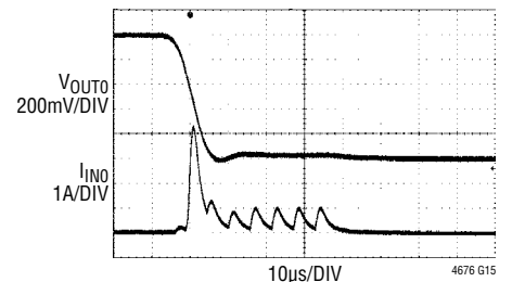
FIGURE 44 CIRCUIT AT 12\text{V}_{\text{IN}} , NO LOAD ON V OUT0 PRIOR TO APPLICATION OF SHORT CIRCUIT
