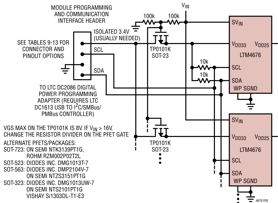
Figure 5. LTM4676 Connection Suitable for Programming NVM of Up to 16 LTM4676s When V IN Power is Absent, 0°C < T J ≤ 85°C
