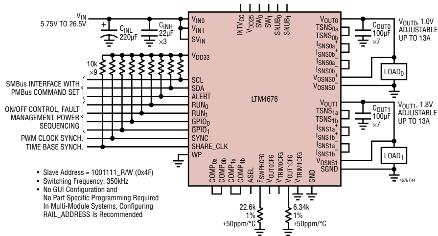
Figure 44. 13A, 1V and 13A, 1.8V Output DC/DC μModule Regulator with Serial Interface
