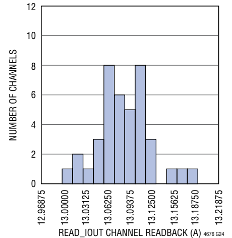
READ_OUT of 20 LTM4676s (DC1811) 12V_{IN} , 1V_{OUT} , T_J = 125^\circ\text{C} , I_{OUTn} = 13\text{A} , System Having Reached Thermally Steady-State Condition, No Airflow
