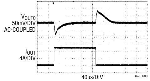
FIGURE 44 CIRCUIT AT 12\text{V}_{\text{IN}} 0A TO 10A LOAD STEP AT 10A/μs
