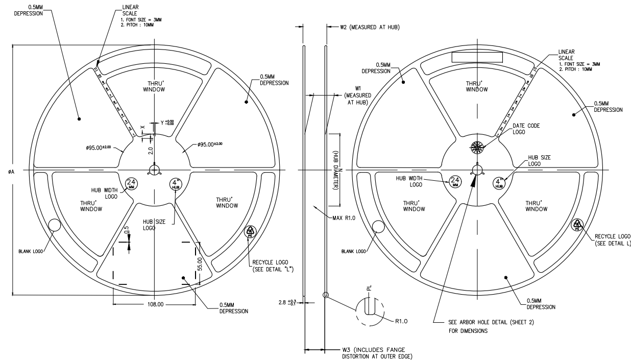
Figure A-4. 212-Ball BGA ZAD Package Plastic Reel
