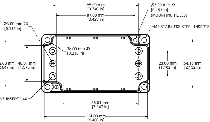
BOX - INSIDE
