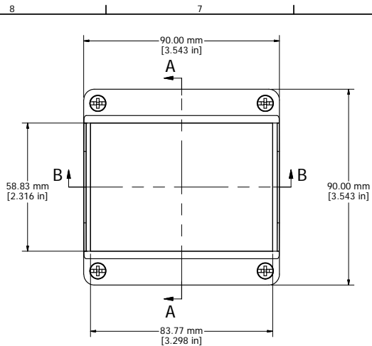
ASSEMBLY
