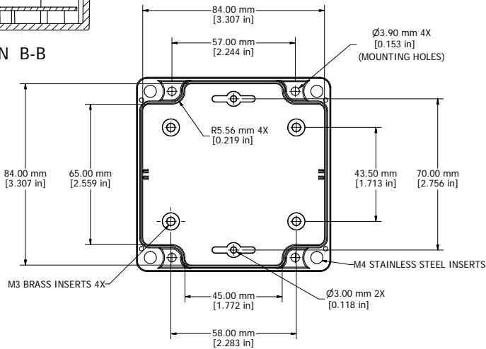
BOX - INSIDE
