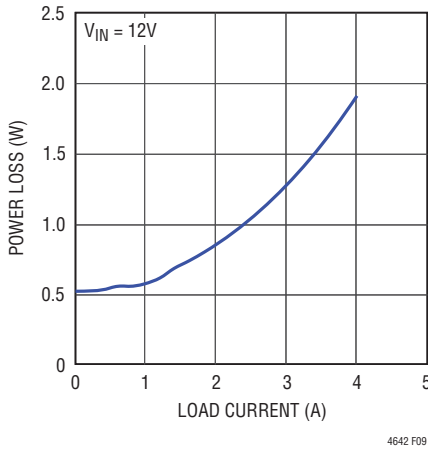
Figure 9. 5V Loss
