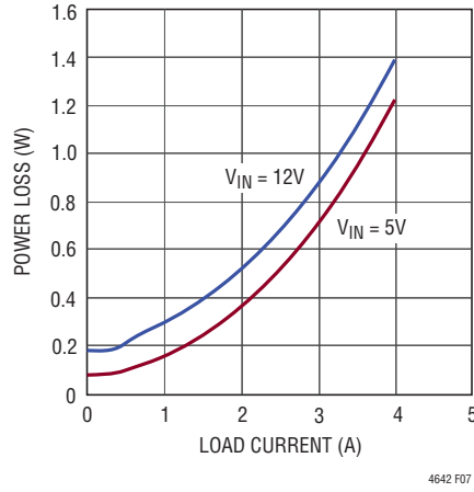
Figure 7. 1.5V Loss
