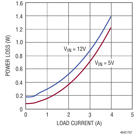
Figure 8. 3.3V Loss
