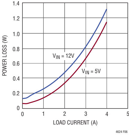
Figure 6. 1.0V Loss
