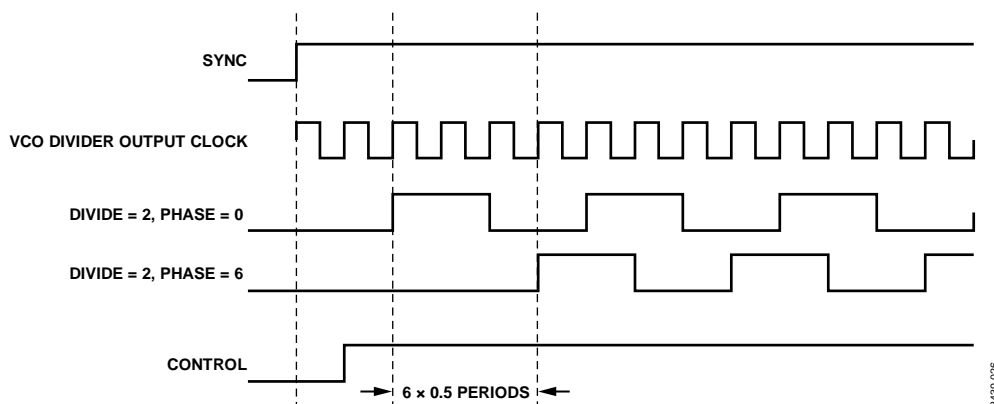
Figure 28. Clock Output Synchronization Timing Diagram
