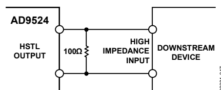
Figure 20. DC-Coupled HSTL Output Driver
