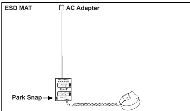
Figure 4. Operating the Jewel® Workstation Continuous Mini Monitor.
