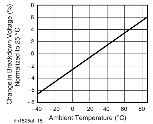
Fig. 16 - Switch Breakdown Voltage vs. Temperature
