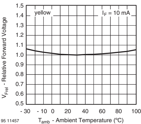
Fig. 15 - Relative Forward Voltage vs. Ambient Temperature
