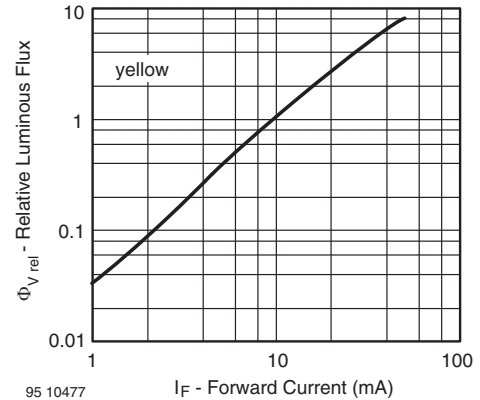
Fig. 16 - Relative Luminous Flux vs. Forward Current
