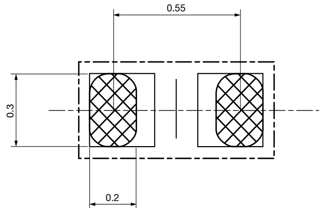
Fig. 2 - Maximum Stencil Openings - for a Stencil Thickness of 80 μm
