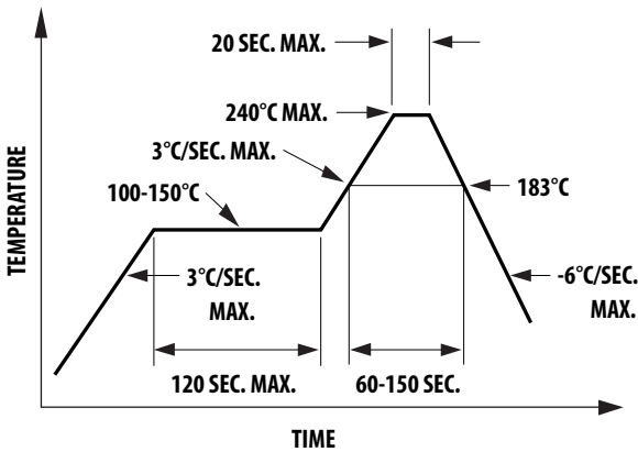
Figure 16. Recommended Leadless Reflow Soldering Profile
