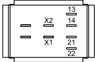
11 Switching element for Pushbutton | Keylock- and Selector switch 2 positions page 35
