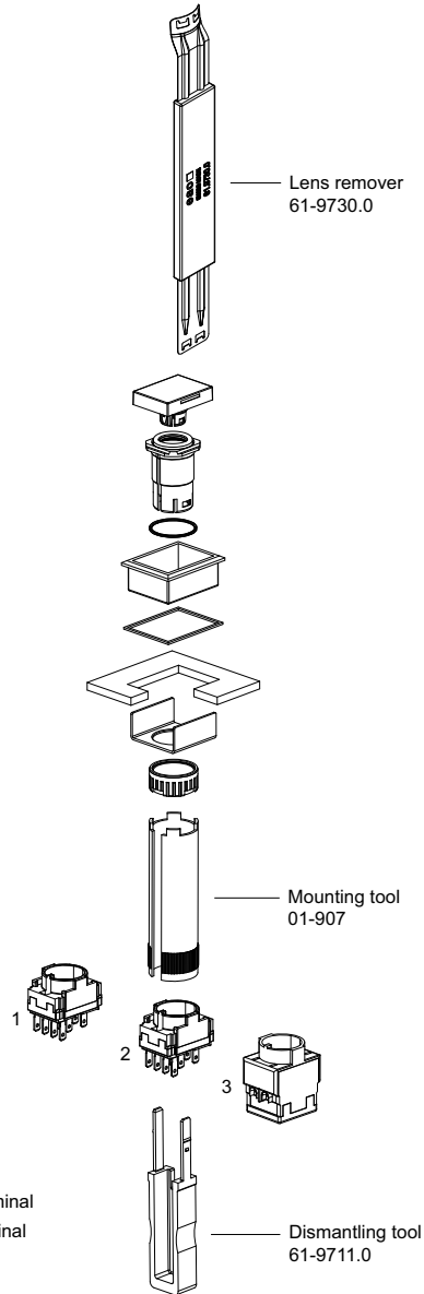
flush mounting
