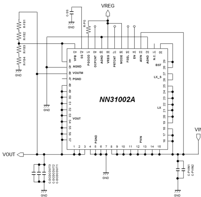
Figure Application circuit
