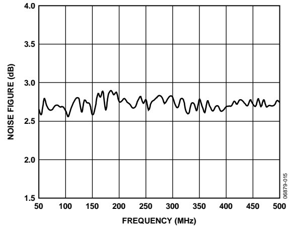
Figure 16. Noise Figure vs. Frequency
