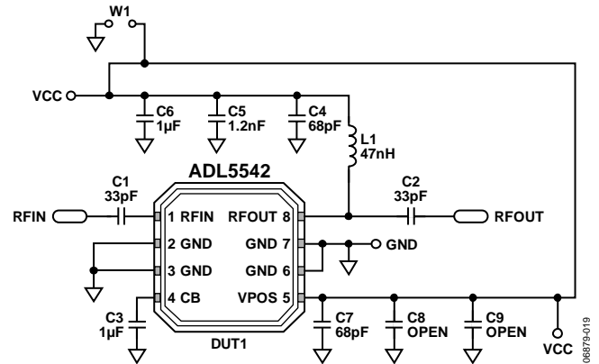
Figure 20. Evaluation Board Schematic
