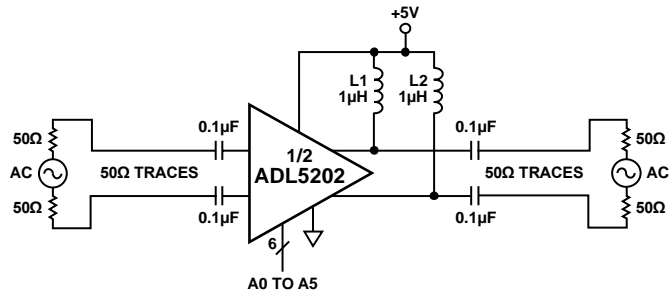
Figure 47. Test Circuit for S-Parameters on Dedicated 50 Ω Differential-to-Differential Board
