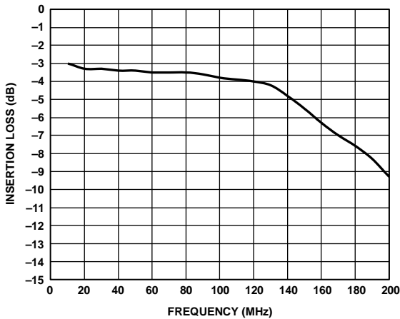
Figure 56. Measured Frequency Response of Wideband ADC Interface, as Depicted in Figure 55
