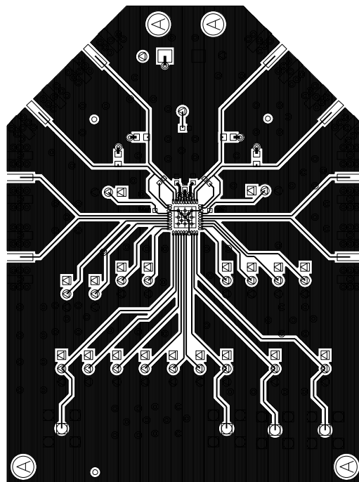
Figure 49. Differential-to-Differential Characterization Board, Circuit Side Layout
