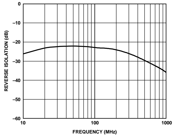
Figure 45. Disable-State Reverse Isolation vs. Frequency
