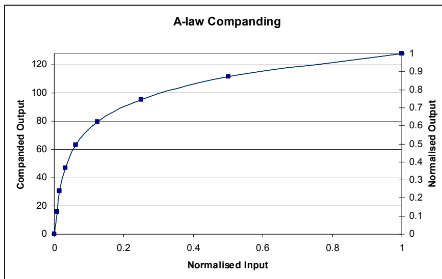
Figure 57 A-Law Companding
