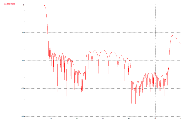
Figure 78 DAC Filter Response for 16k Sample Rate
