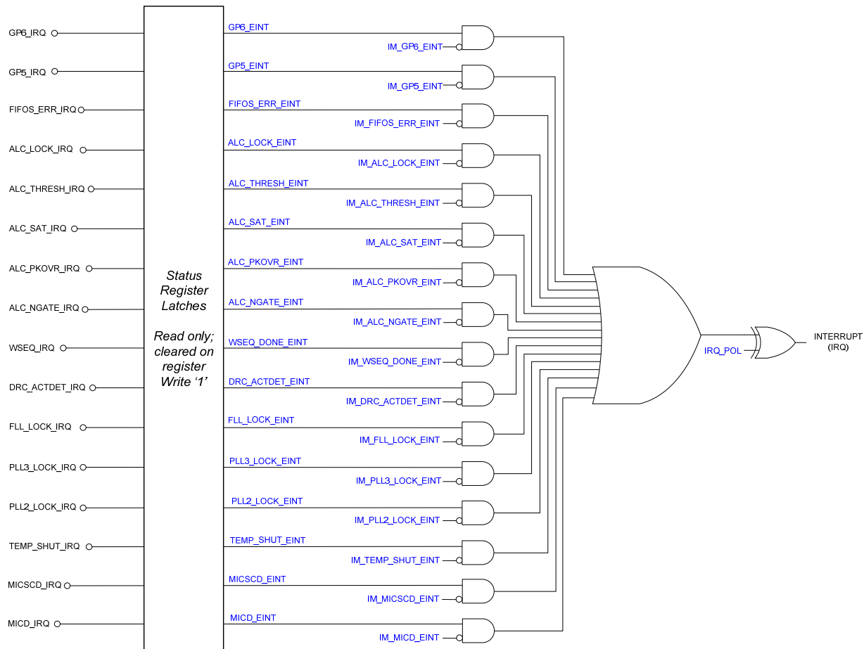
Figure 63 Interrupt Controller
