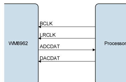
Figure 40 Slave Mode
