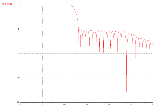
Figure 83 DAC Playback Filter Response for 48k Sample Rate
