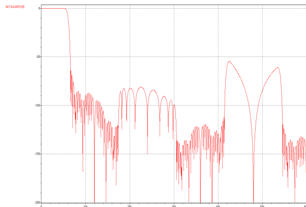
Figure 77 DAC Filter Response for 12k Sample Rate
