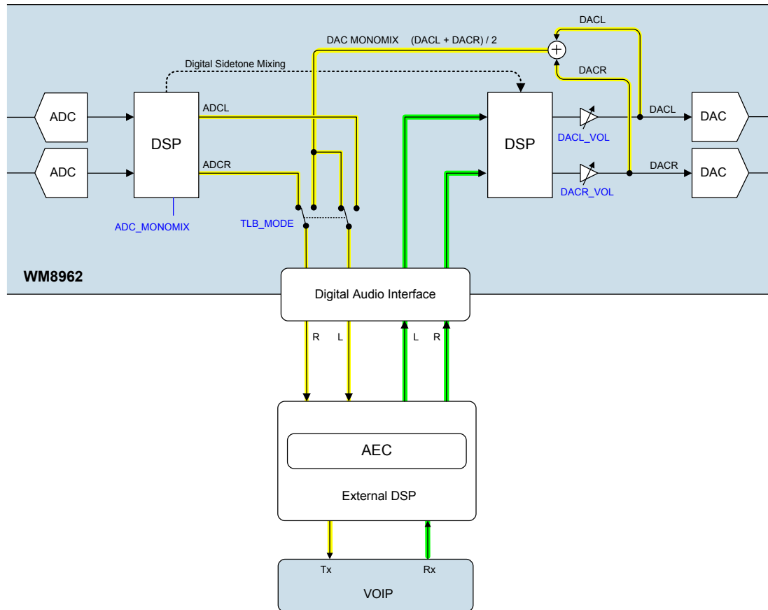
Figure 31 T-Loopback Signal Paths
