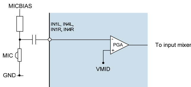
Figure 14 Microphone Input IN1 or IN4
