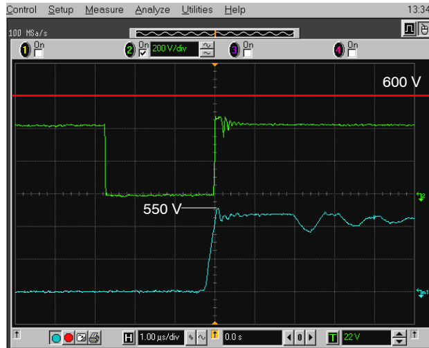
Figure 10. Maximum Output Power, V_{in} = 265 \text{ Vac} Note the good margin on the drain thanks to the low leakage term
