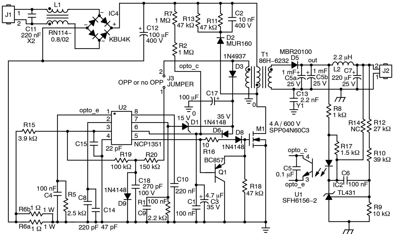
Figure 3. The 57 W Adapter Board Featuring the NCP1351 Controller
