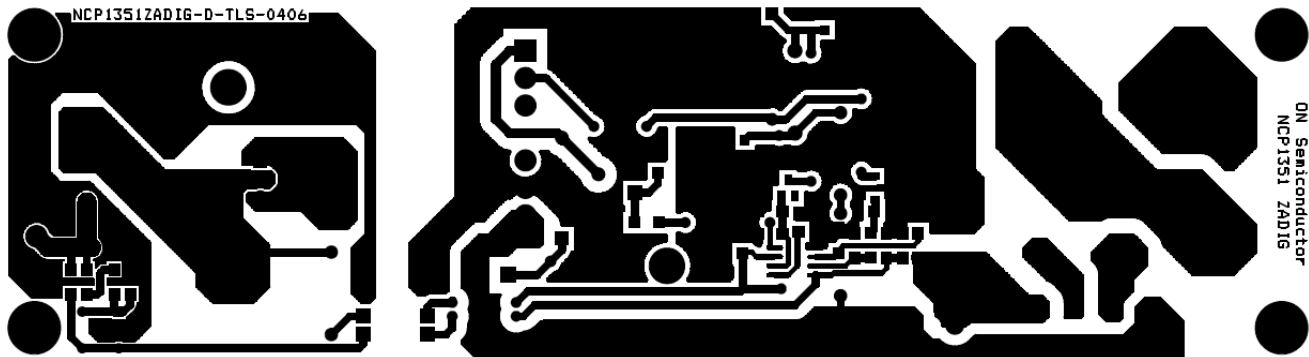
Figure 17. Copper Traces
