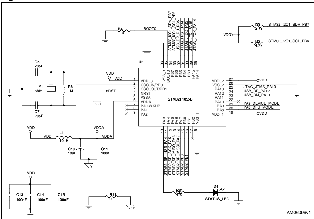
Figure 2. Microcontroller section
