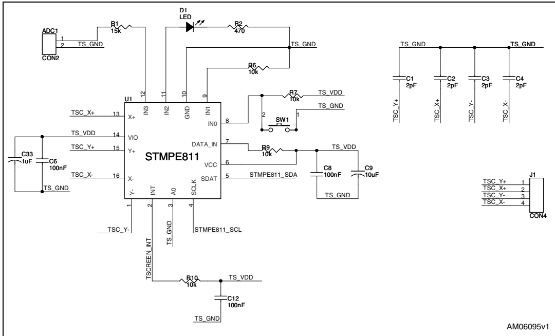
Figure 1. Touchscreen controller
