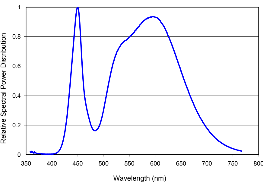
Figure 9. Color spectrum of LXH7-PW40 emitter, integrated measurement.
