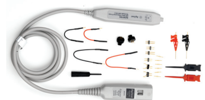
N2819A 800-MHz, 15-V differential probe with AutoProbe interface
