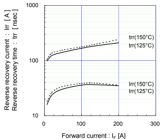
Reverse recovery characteristics (typ.) Vcc=300V, VGE=±15V, Rg=13Ω
