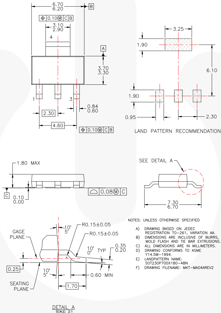
Figure 14. MOLDED PACKAGE, SOT-223, 4 LEAD (ACTIVE)
