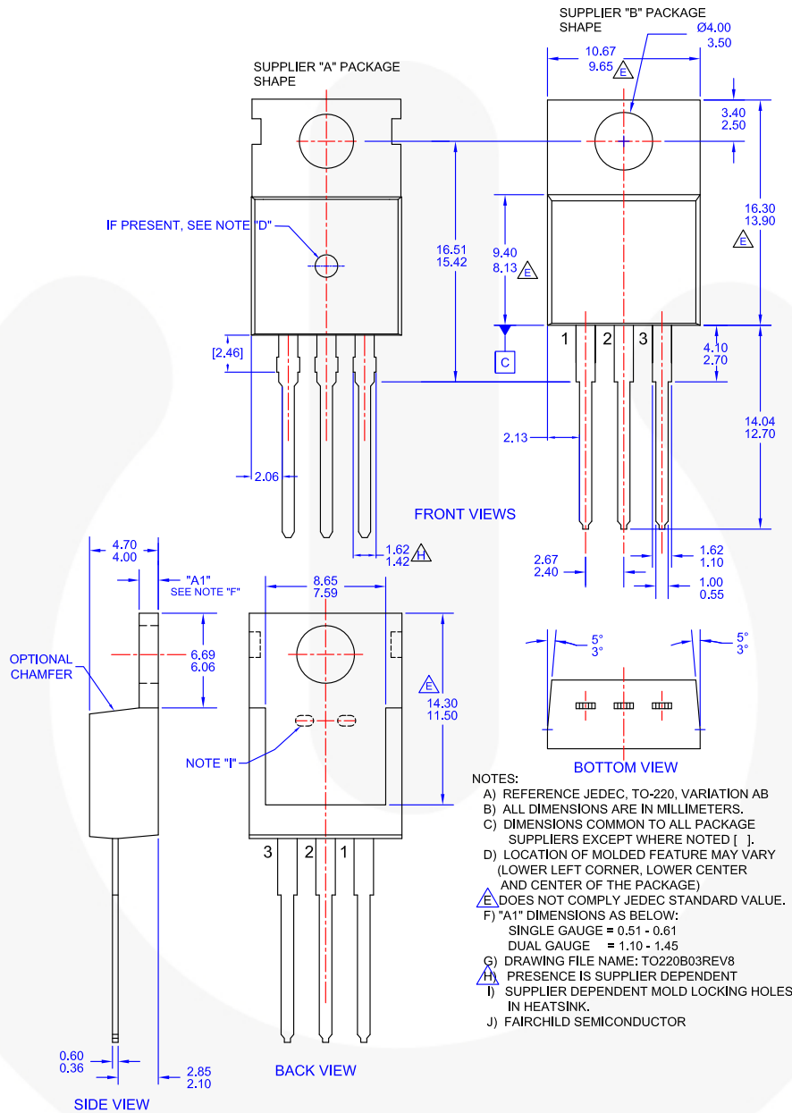
Figure 13. TO-220, MOLDED, 3LEAD, JEDEC VARIATION AB (ACTIVE)
