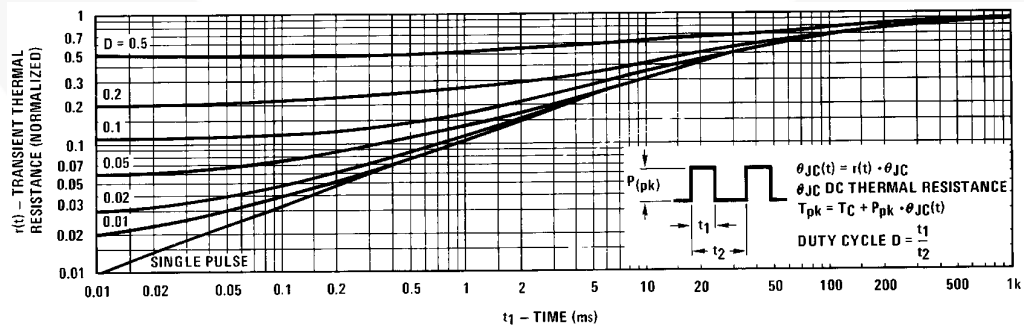
Figure 12. Thermal Response in TO-220 Package
