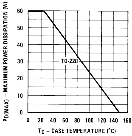
Figure 9. Maximum Power Dissipation vs. Case Temperature
