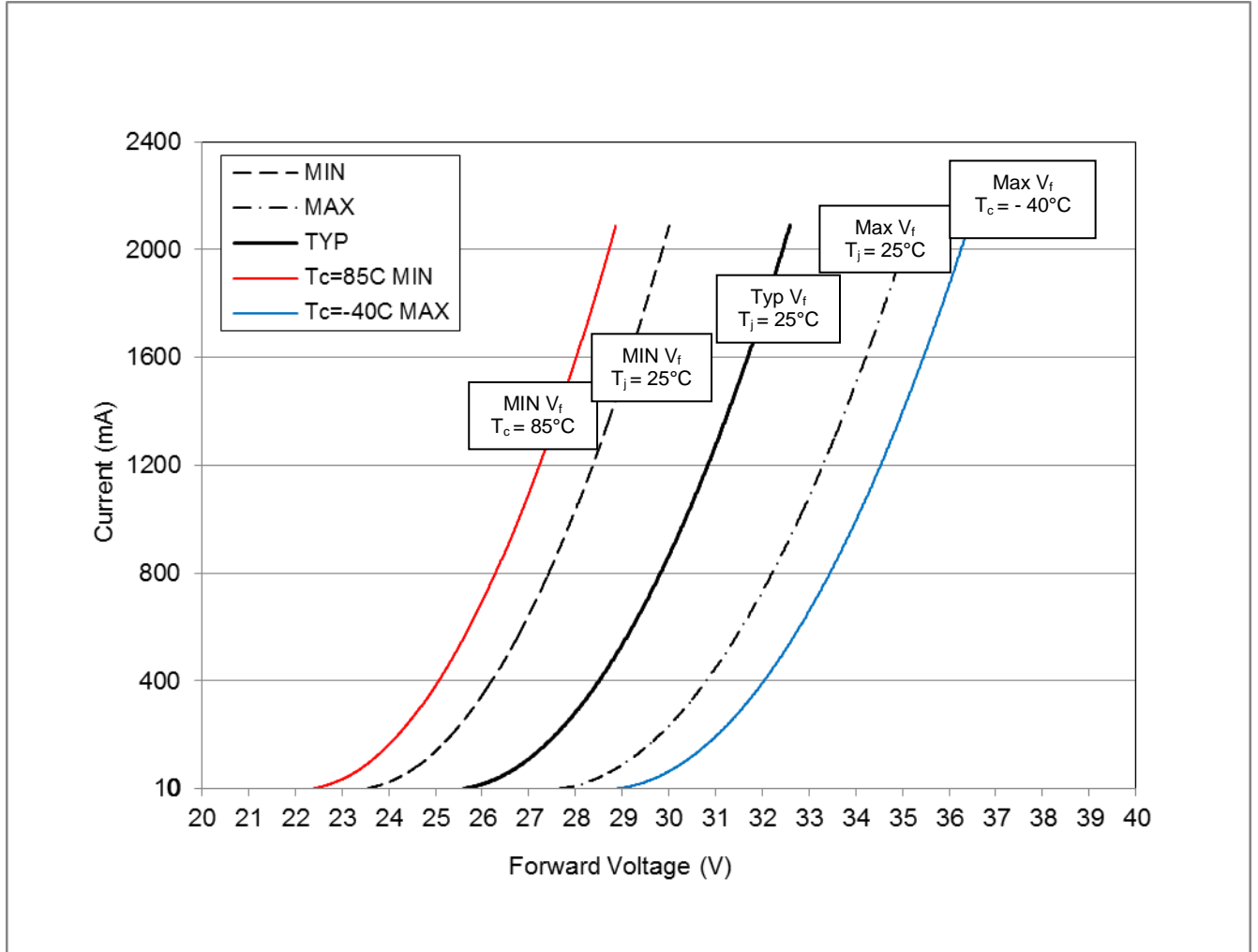
Figure 1: Electrical Characteristics
