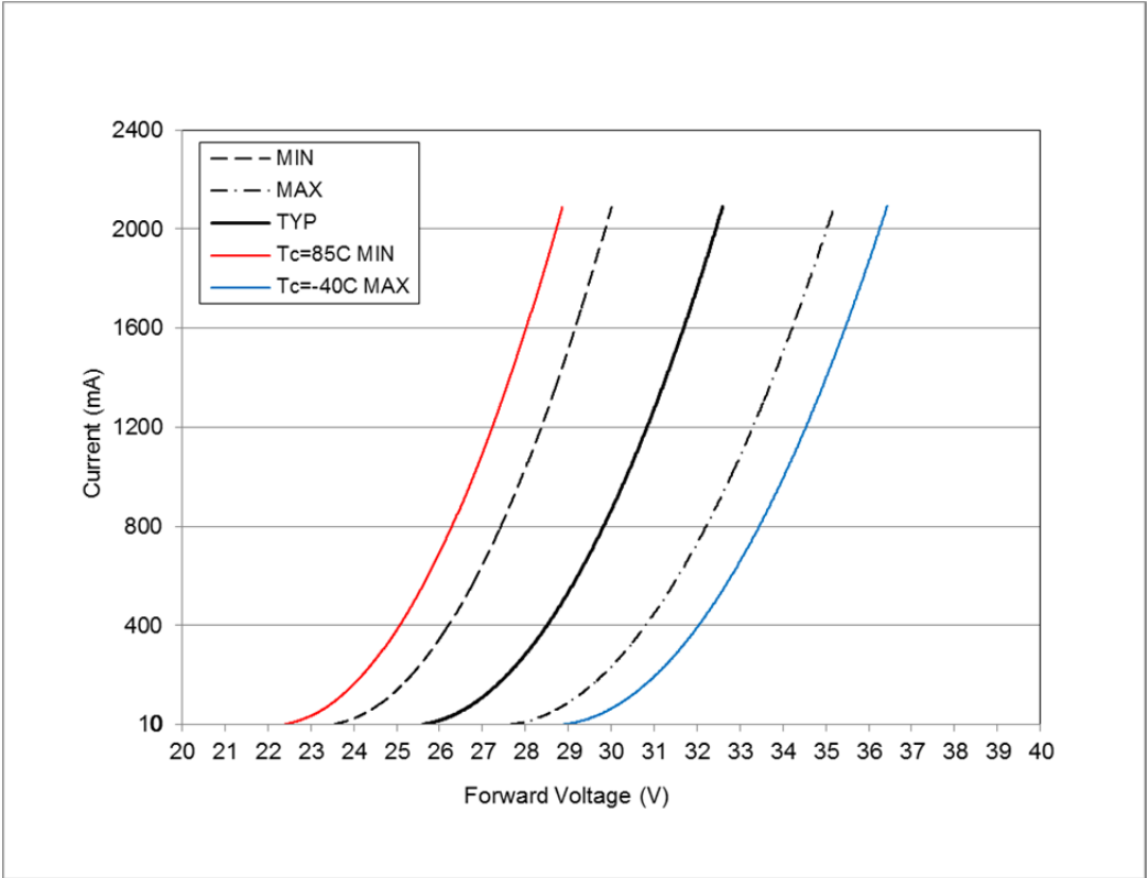
Figure 1: Typical Drive Current vs. Voltage
