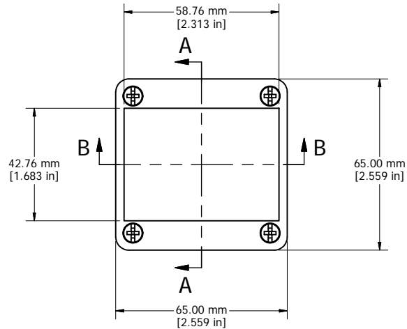
ASSEMBLY
