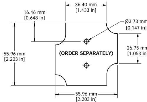
STEEL INNER PANEL
