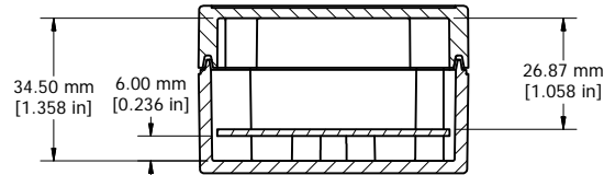
SECTION B-B
