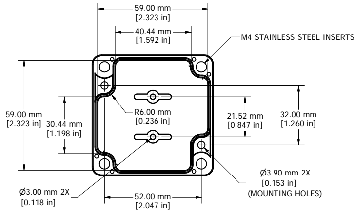
BOX - INSIDE
