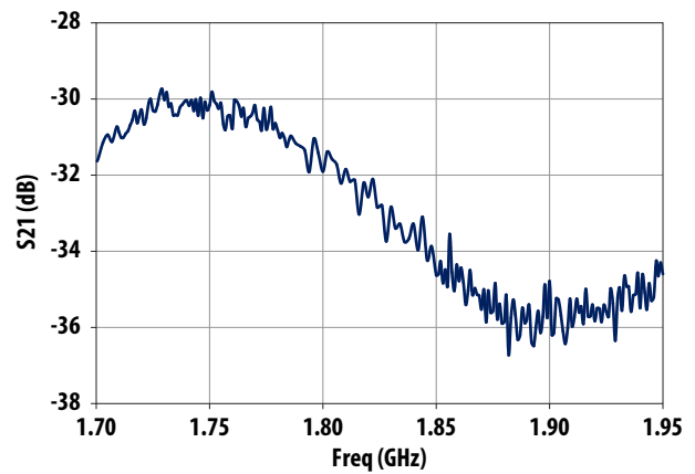
Figure 6d. S21 plot for (1700 - 1950) MHz
