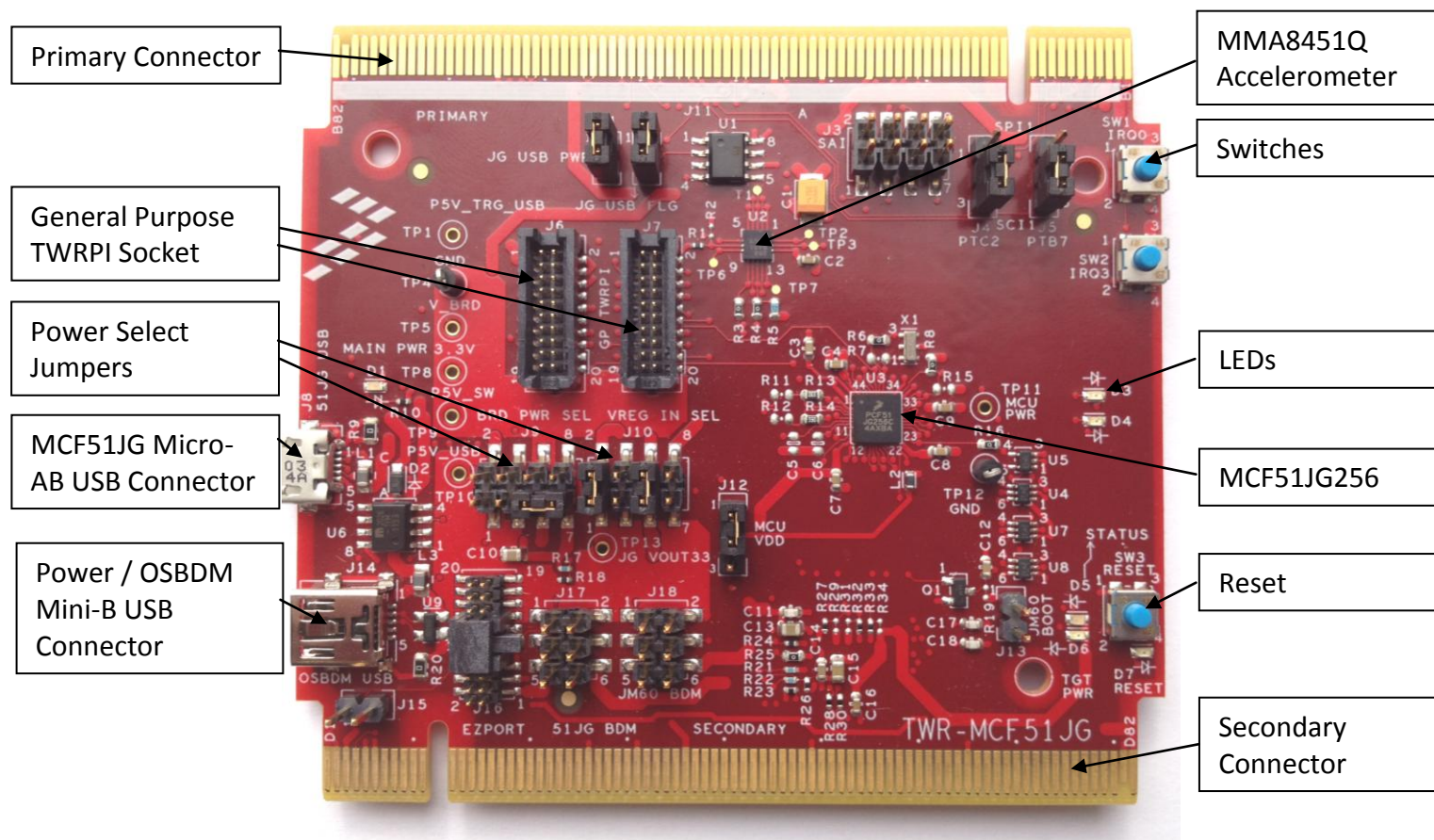
Figure 2. Callouts on front side of the TWR-MCF51JG
