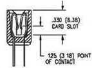
INSULATOR STYLE CODE 5
