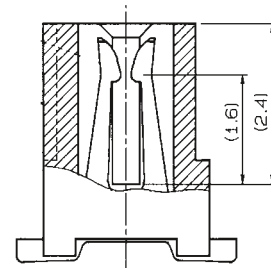
SECT. X-X
