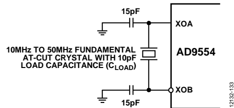
Figure 24. System Clock Input (XOA/XOB) in Crystal Mode (The capacitor values shown are for a crystal with a C_{LOAD} = 10\text{ pF} . The values of 15 pF shunt capacitors shown here must equal 2 \times (C_{LOAD} - C_{STRAY}) , where C_{STRAY} is typically 2 pF to 5 pF.)
