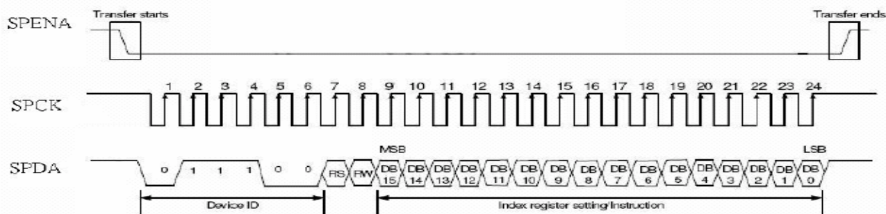
Figure12 SPI timing
